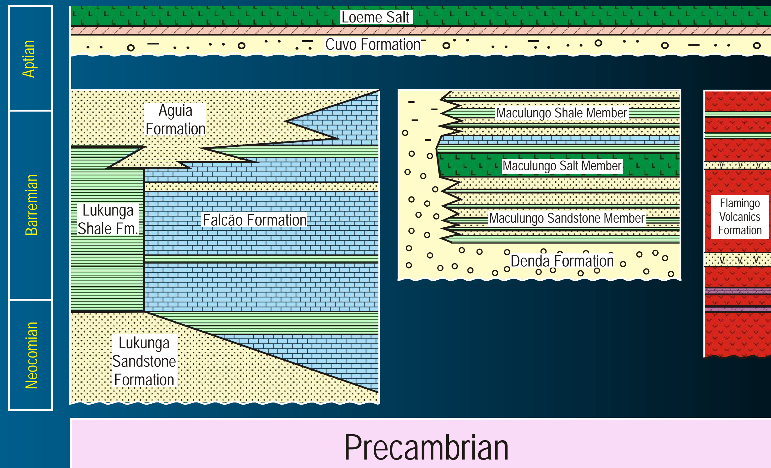
PROPOSED PRE-SALT LITHOSTRATIGRAPHY
