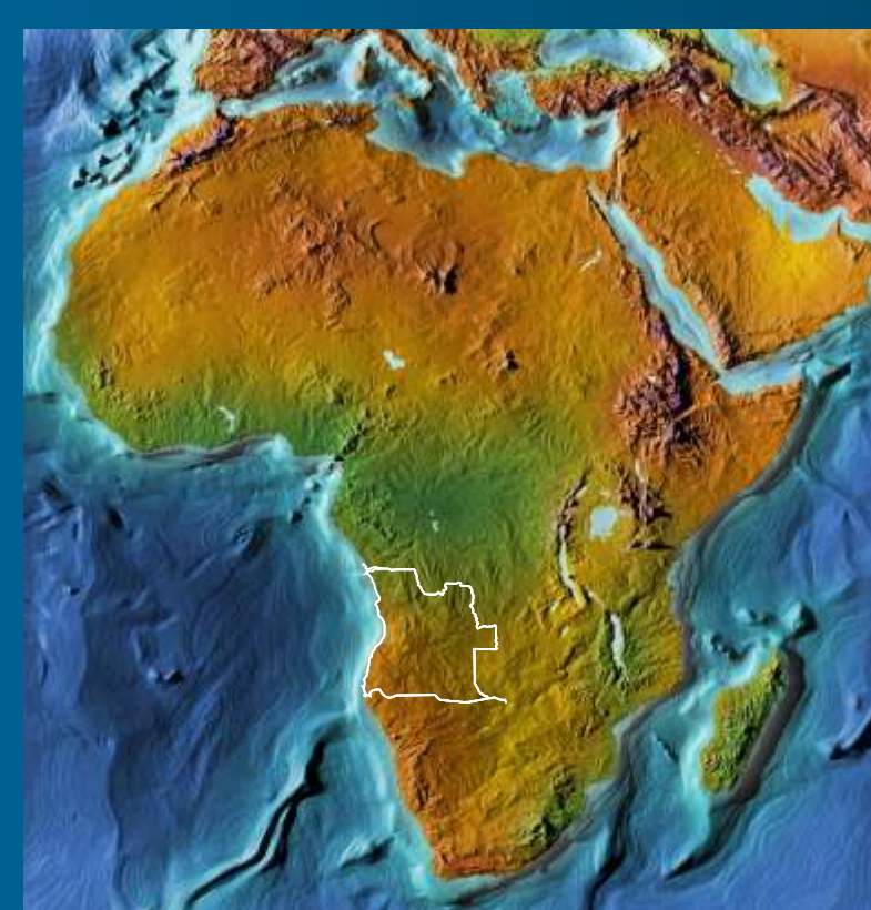
Kwanza Basin, Angola
