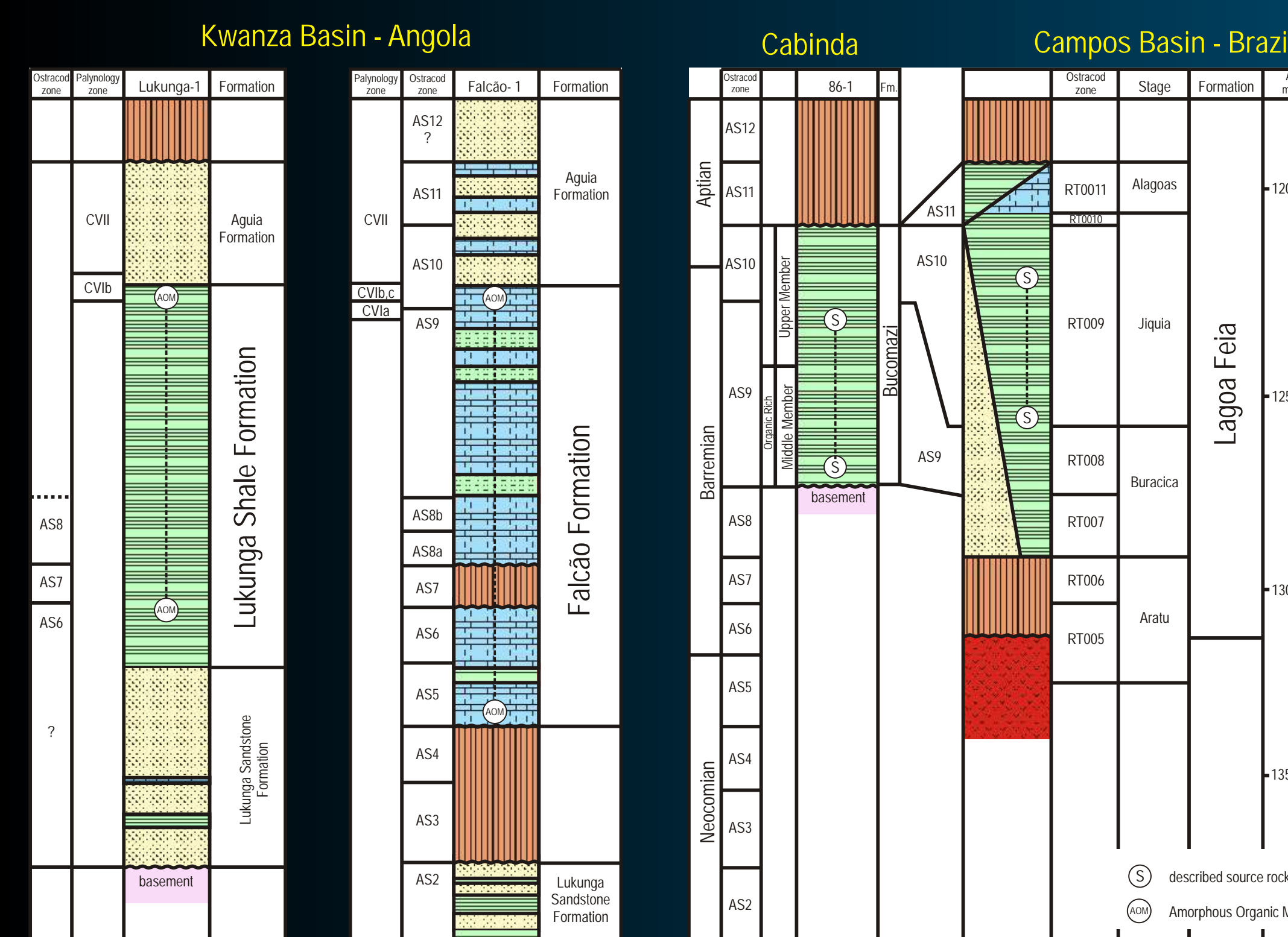
THE REVISED LUKUNGA-1 / FALCÃO-1 AGE RELATIONSHIP AND THE TIES TO CABINDA AND CAMPOS BASIN SOURCE HORIZONS
